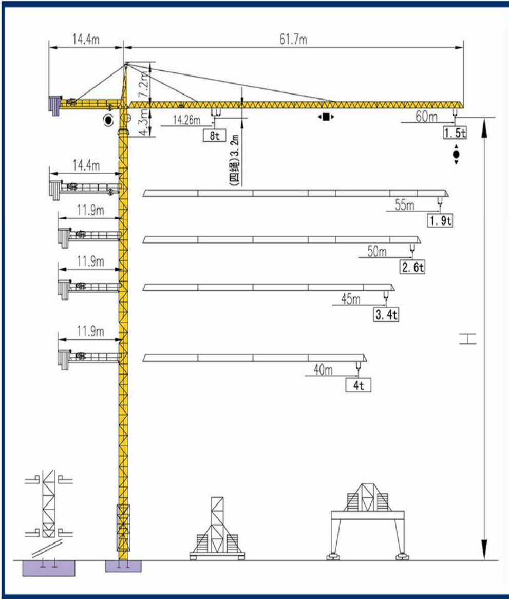
TOWER CRANE (QTZ 115tm)
