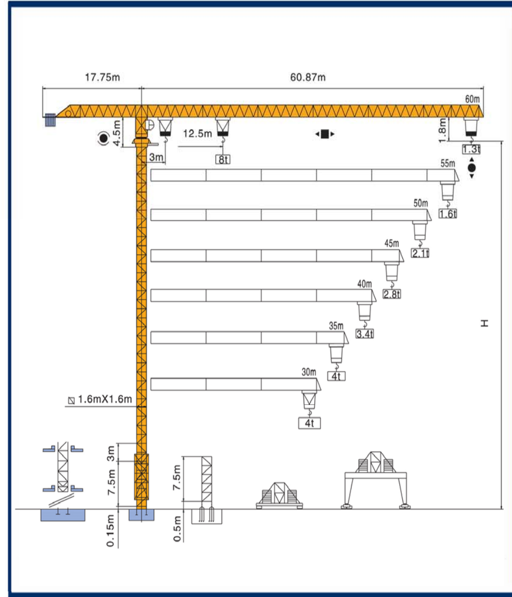
TOWER CRANE (QTP 140tm)
